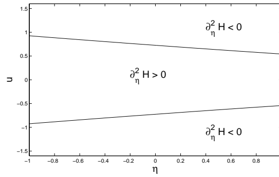
Figure 1. Regions of phase space (\eta, u) where \partial_{\eta}^2 H < 0 and \partial_{\eta}^2 H > 0 . The parameters are h = h_1 = 1 , \rho = 1 and \rho_1 = 0.7 .
