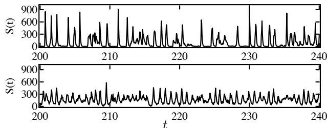
FIG. 4.1. The bulk synaptic output function S(t) ; one trial each for the two sets of parameters in figure 3.1.
